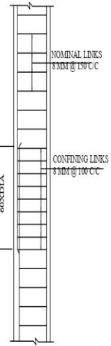
LAP / SPLICE IN COLUMN MAY BE PROVIDED IN THE MIDDLE PORTION OF COLUMN
