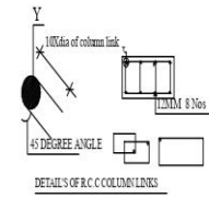
DETAILS OF R.C.C. COLUMN LINKS
