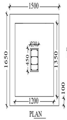
DETAILS OF R.C.C. BOX FOOTING COLUMN NO. C1
