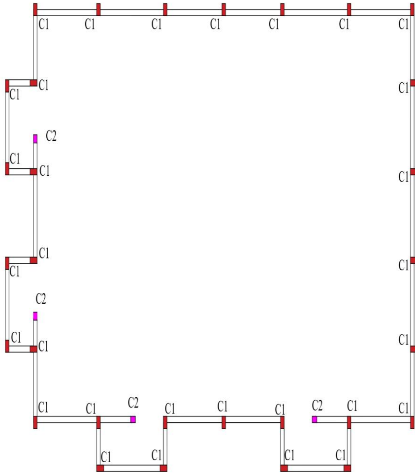
LAP / SPLICE IN COLUMN MAY BE PROVIDED IN THE MIDDLE PORTION OF COLUMN
